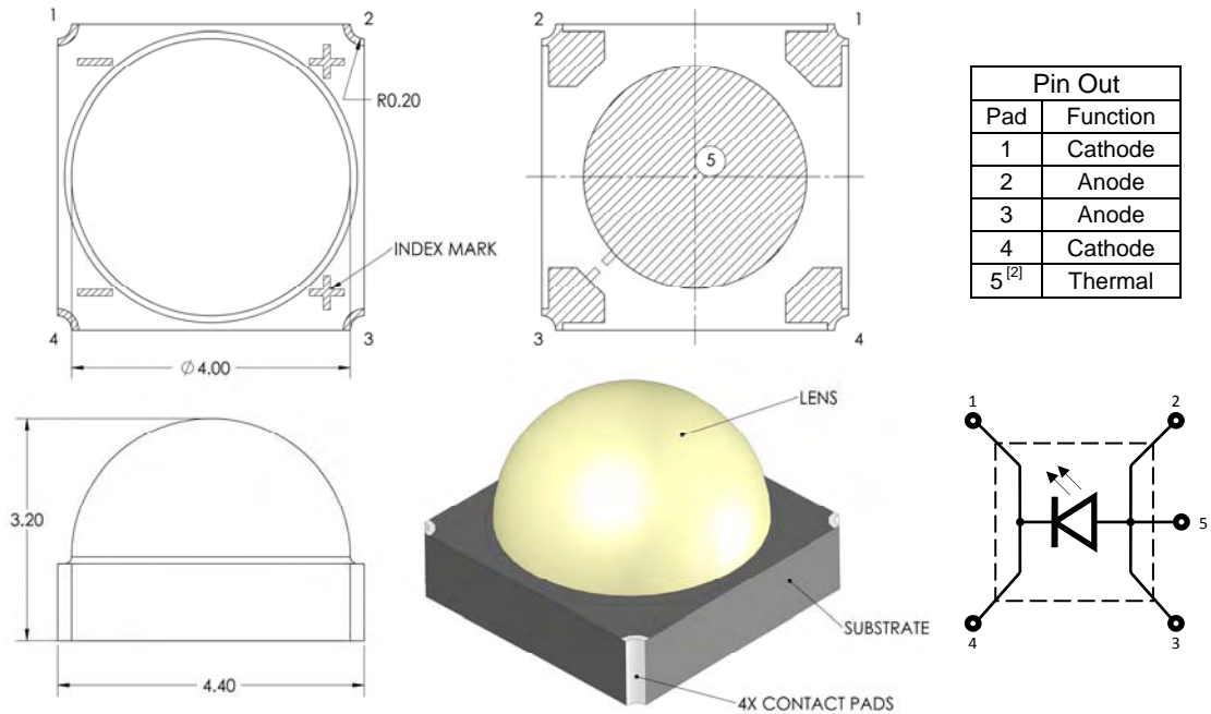
Figure 1: Package outline drawing.
